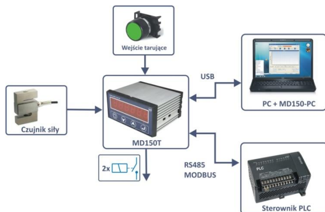
Picture. 1 Example of MD150T external connections.
